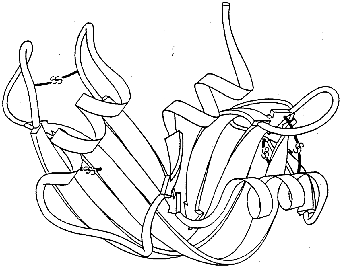
Ribonuclease A
