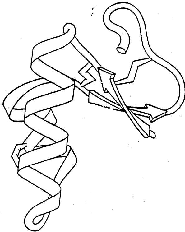
Crambin
